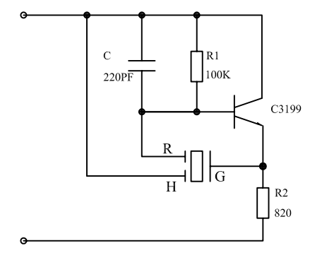
Test Circuit
